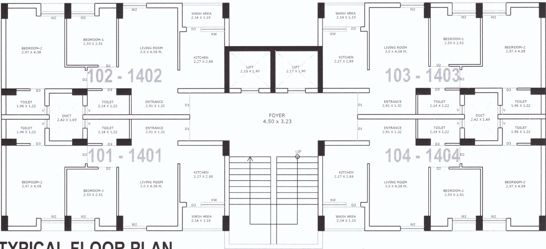
TYPICAL FLOOR PLAN (1st to 14th)_Building No.1
