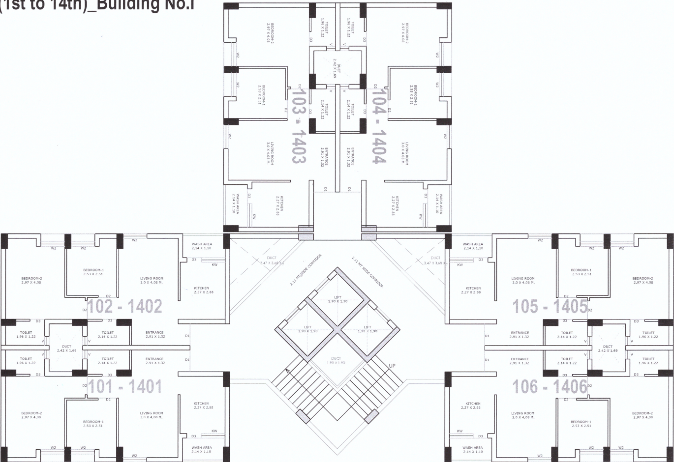
TYPICAL FLOOR PLAN (1st to 14th)_ Building No.A,B,C,D,E,F,G,H
